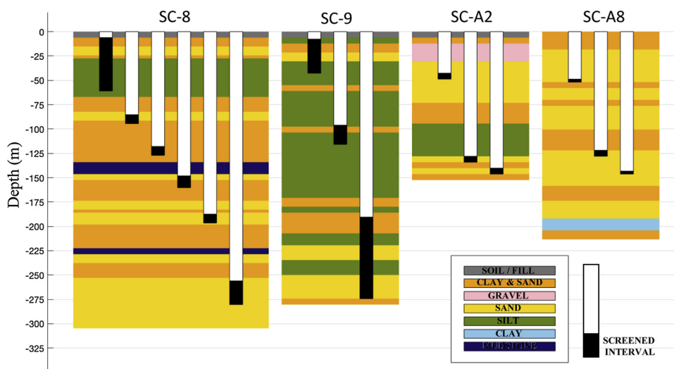
Fig. 3. Schematic of the four Soquel Creek nested monitoring well sets used for developing the resistivity-to-water-quality transform. The lithology for each well set, taken from the driller's lithologic log, is shown in color, overlain by each well in the nested set with the well's screened interval shown in black. Locations of these wells are noted in Fig. 1c.
