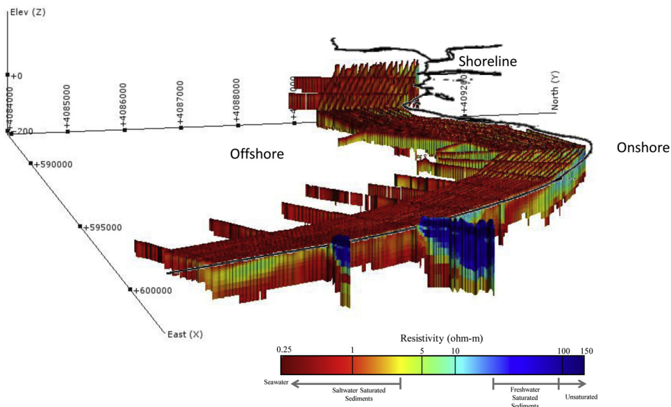
Fig. 8. Three-Dimensional view of the inverted resistivity models, for all values above 0.3 ohm-m (removes the seawater layer). Data are masked below the DOI. The shoreline, taken from where the DEM hit 0 mbsl, is marked with a black line.
