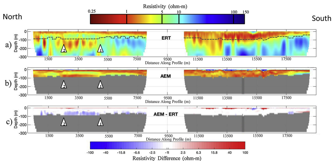
Fig. 7. Comparison of ERT and AEM datasets along the coast of the Salinas Valley area, with the ERT profile in 7a, nearest AEM data mapped onto the ERT profile in 7b, and the difference between the two (AEM-ERT) in 7c. The dashed line on the ERT profile represents the DOI of the AEM profile. Both AEM profile, and the difference profile are gray below the DOI of the AEM dataset.
