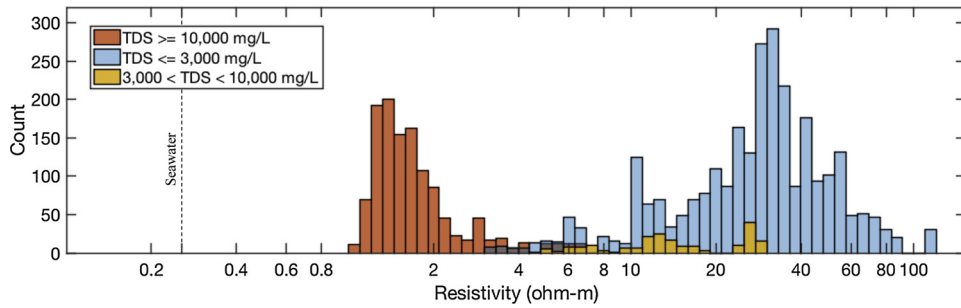
Fig. 5. Combined histograms of the well log resistivity measurements from the Soquel Creek and Salinas Valley regions, colored according to the TDS measurement made within the screened intervals matching the depths of the resistivity values. The annual mean seawater resistivity taken from the MBARI C1 monitoring site is noted with a dashed line at 0.256 ohm-m.
