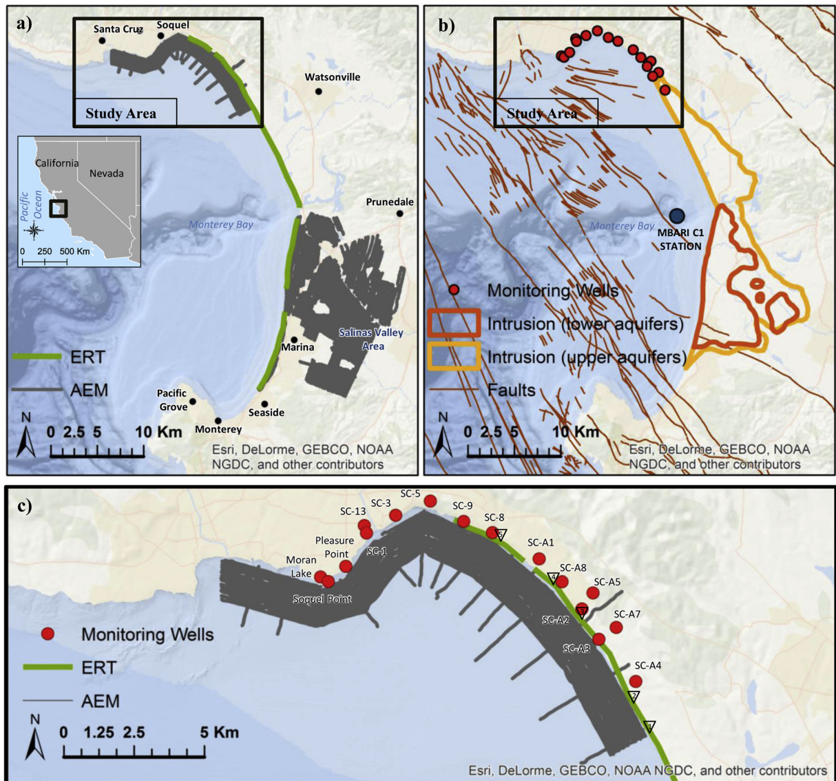
Fig. 1. Location of the study area within the greater Monterey Bay Region: a) showing locations of AEM data (in gray) for this study and in the Salinas Valley area from Gottschalk et al. (2018) , ERT data from Goebel et al. (2017) in green, and the outline of the groundwater basins in the region in tan (DWR, 2017); b) showing locations of the monitoring wells closest to the coast within the study area in yellow, large rivers and streams in blue, faults in red, and the extent of saltwater intrusion in the upper aquifers in light orange, the extent of intrusion in the deeper 400 ft aquifer in dark orange, and the location of the Monterey Bay Aquarium marine monitoring station C1 in blue; c) showing a zoomed in view of just the study area showing the spatial relationship between the AEM data, ERT data, and monitoring wells discussed in the text, with names displayed next to the monitoring wells, and triangular markers along the ERT data marking points discussed in the text (For interpretation of the references to colour in this figure legend, the reader is referred to the web version of this article).
