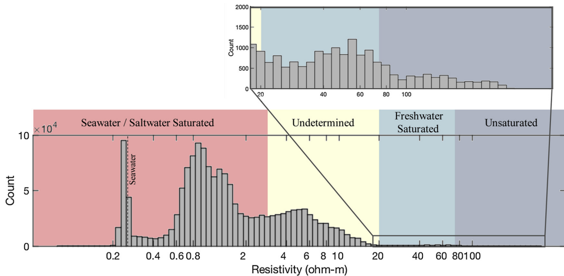
Fig. 6. A histogram of resistivity values resulting from the inversion of the AEM dataset, annotated with the water quality transform established using well data. The annual mean seawater resistivity taken from the MBARI C1 monitoring site is noted with a dashed line at 0.256 ohm-m. An enlarged view of the highest resistivity values is shown above the primary figure.
