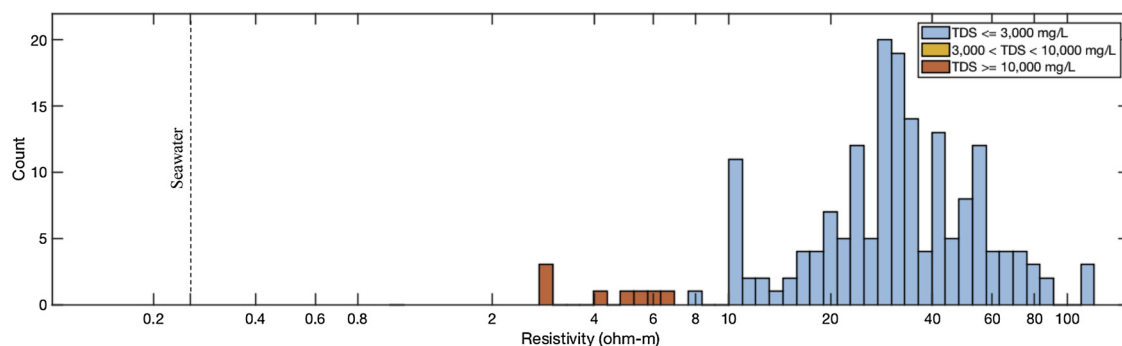
Fig. 4. Histograms of resistivity measurements sampled from the resistivity logs every 1.5 m within the screened intervals in Soquel Creek coastal monitoring wells, colored according to the TDS measurement made within that screened interval. The annual mean seawater resistivity taken from the MBARI C1 monitoring site is noted with a dashed line at 0.256 ohm-m.
