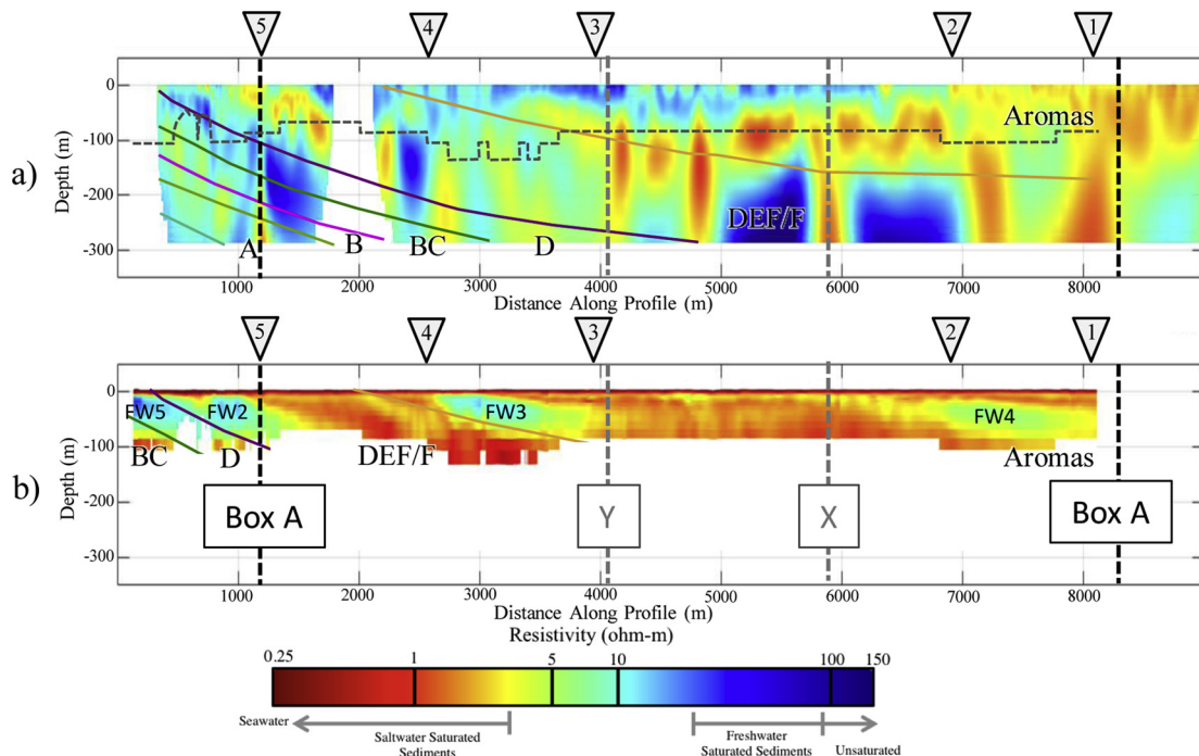
Fig. 11. Inverted resistivity from ERT data collected along the beach (a), and inverted resistivity from the closest offshore AEM flight line (b). The dashed gray lines mark the intersection of the cross sections shown in Figs. 10a and b with these two profiles, and the dashed black lines mark the boundaries of Box A in Fig. 9. Hydrostratigraphic unit boundaries are marked, and markers 1–5 at the top of the figures note locations referenced in the discussion of this figure. Markers ‘FW2–5’ reference locations discussed in the text.
