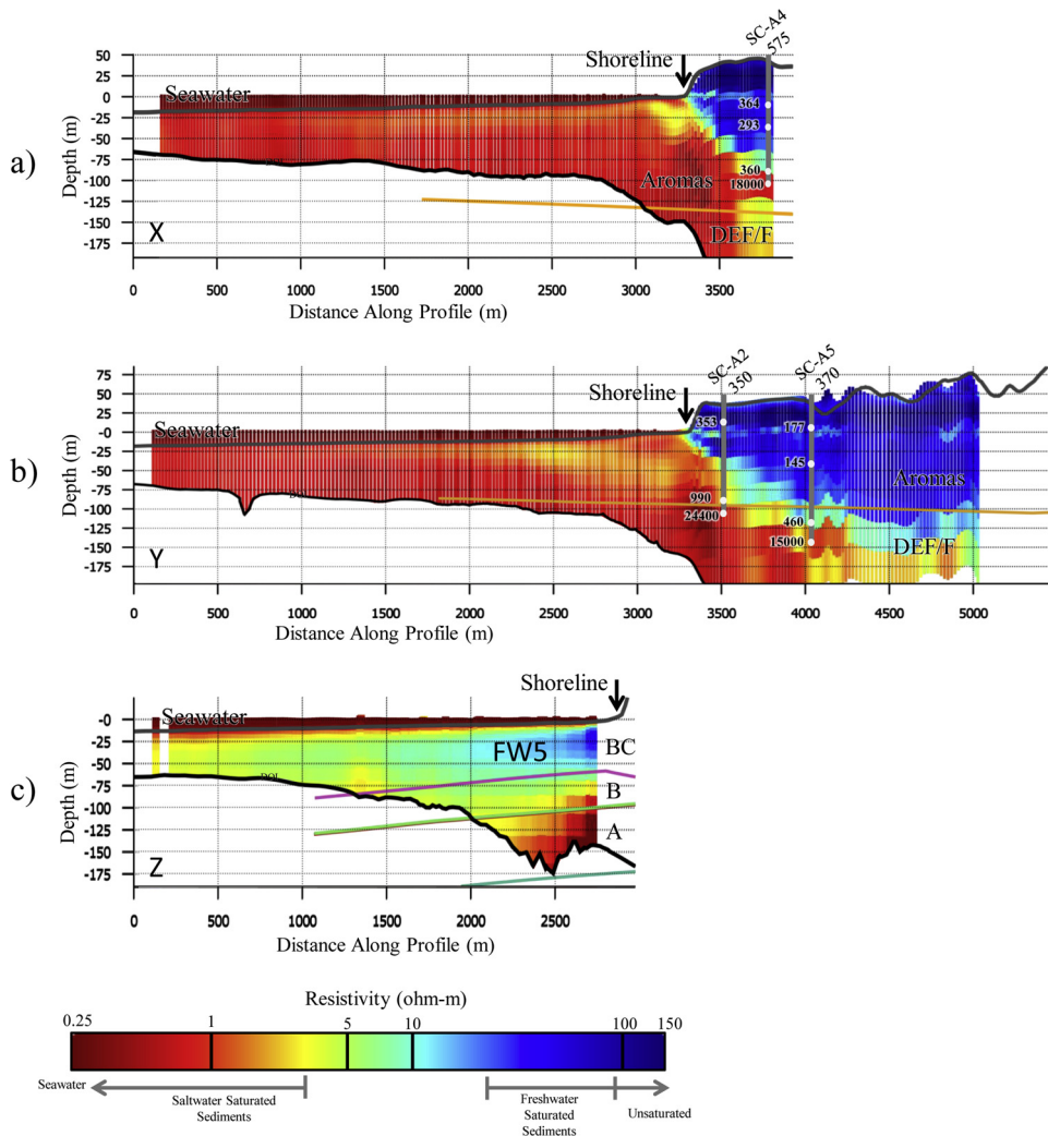
Fig. 10. Cross sections of the inverted resistivity models along the profiles 'X' (10a), 'Y' (10b), and 'Z' (10c) noted in Fig. 9. Data are masked below the DOI. Hydrostratigraphic boundaries from the groundwater flow model are noted with the same color scheme as in Fig. 9, and units are labeled according to the names given in Table 1. Monitoring wells are projected onto the cross sections, with the 2016 TDS values (in units of mg/l) measured in each of the screened intervals noted next to the depth of that screened interval. The onshore and offshore DEM are noted with a gray line.
