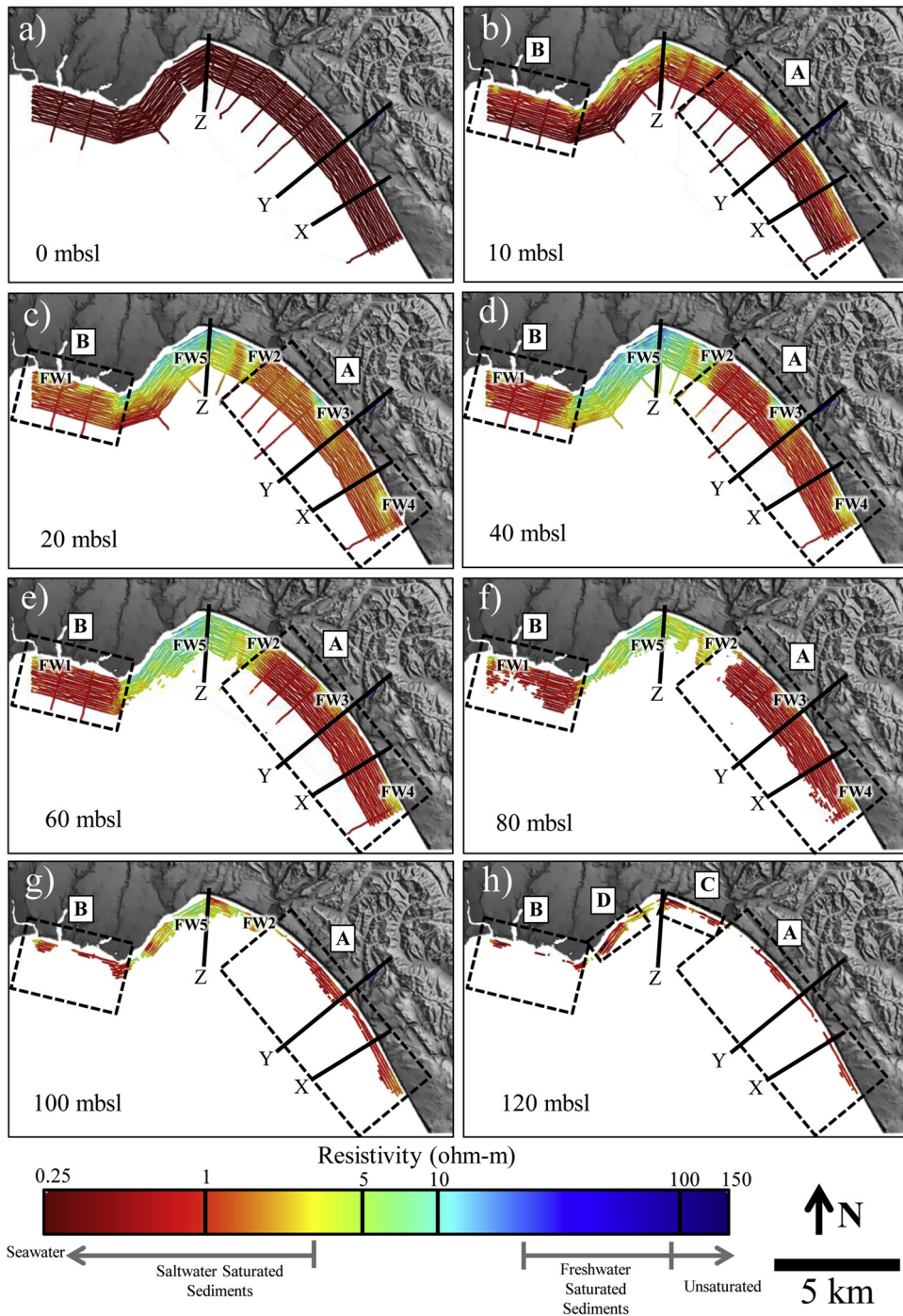
Fig. 9. Depth slices through the inverted resistivity models from 0 to 120 mbsl, next to the shaded DEM onshore. Data are masked below the DOI. Lines, boxes, and numbers on the figures indicate locations or regions that are discussed in the text.
