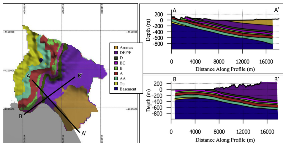
Fig. 2. Hydrostratigraphic boundaries of the groundwater model used for management of groundwater resources in the Soquel Creek Area, viewed in plan view on the left and along two cross sections on the right. The locations of the two cross sections are annotated as lines A/A' and B/B' on the plan view. In plan view, the areas in the figure offshore are marked in transparent gray.
